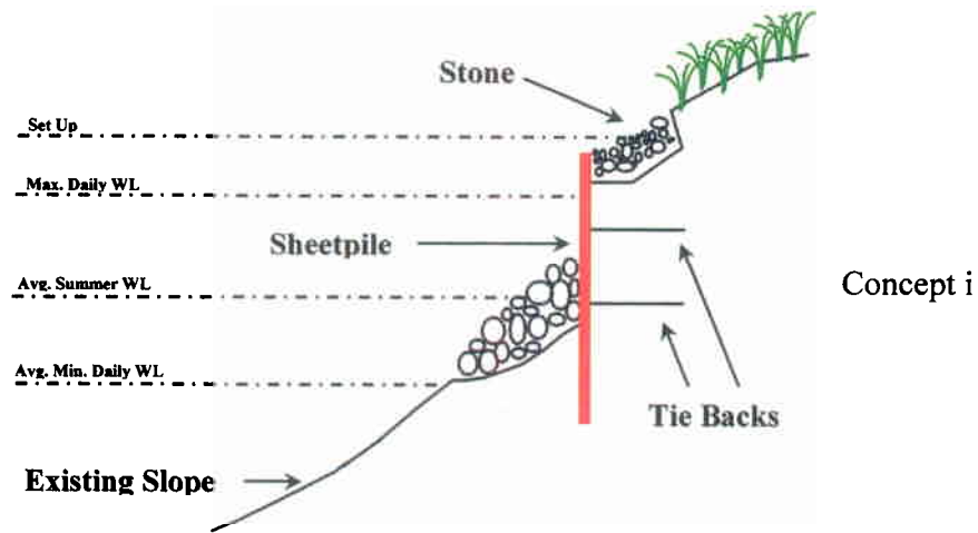
FIGURE 3: CONCEPTUAL SHORELINE DESIGNS FOR SHORELINE AREAS OF SPECIAL CONCERN TO ADJACENT LAND OWNERS (from Baird and Associates, 1999)
